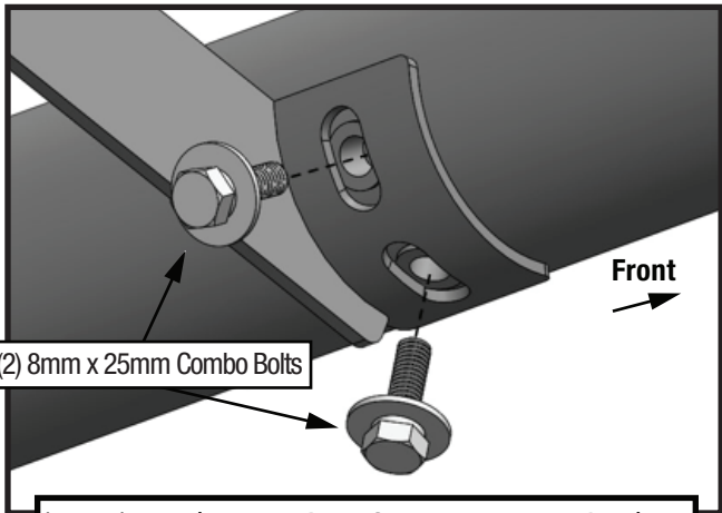
(Fig 14) Attach Access Drop Step to Mounting Brackets
