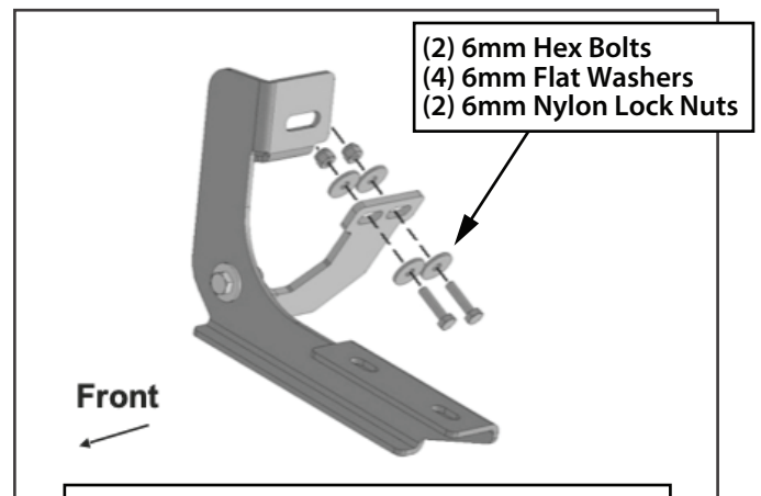
(Fig 14) Attach driver/left center/rear Support Bracket to back of pinch weld (models with factory holes in pinch weld only)
