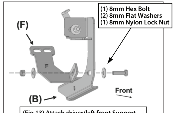
(Fig 13) Attach driver/left front Support Bracket (F) to rear facing side of Mounting Bracket (B)
