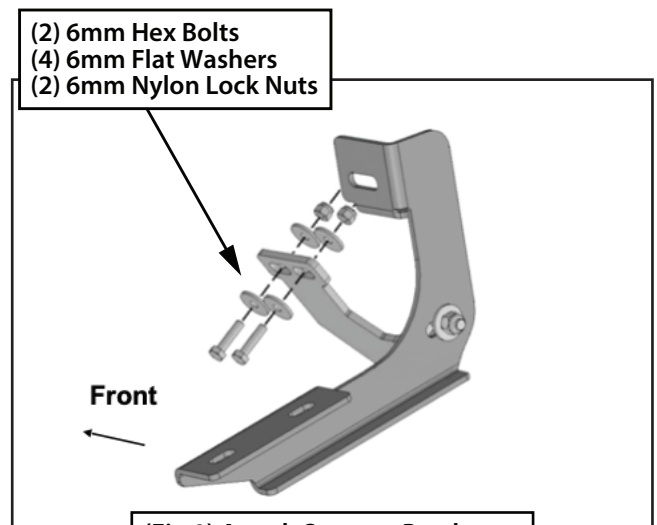
(Fig 9) Attach Support Bracket to back of pinch weld (models with factory holes in pinch weld only)
