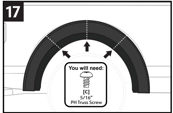
17. While applying pressure to the flare, install a 5/16" Truss Screw [C] through the 3 top flare holes and attach to the S-Clips.
