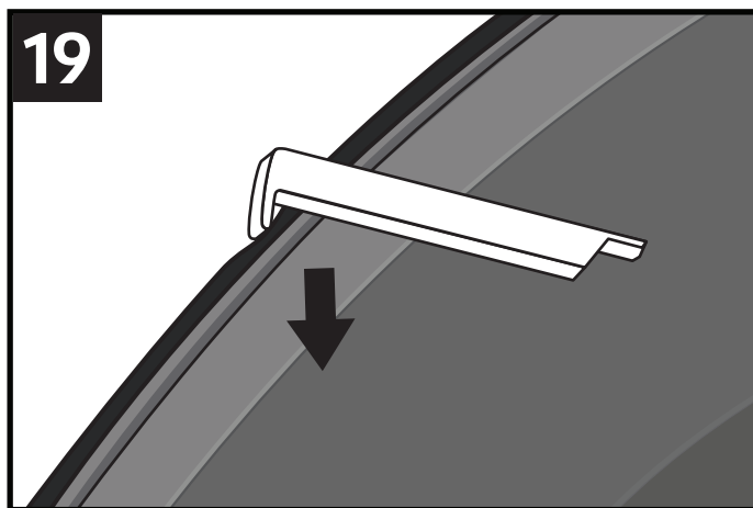
19. If needed, use supplied Edge Trim Tool [H] to trim outer edge by inserting the curved end, then sliding around the entire trim from one end to the other.
