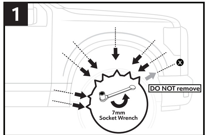
1. With 7mm socket wrench, remove and keep 7 factory screws to be reinstalled later. Note: DO NOT remove the 8th screw as shown.
