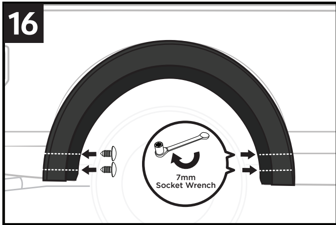
16. Hold up flare again firmly press against the vehicle. Then reinstall the 2 front screws removed from STEP 12 with 7mm socket wrench. Apply 2 Nylon Retainers [G] to the 2 rear bottom holes.
