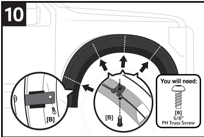
10. Press flare inward and firmly against the body panel and install 4 x 5/8" Truss Screws [B] through the flare and into the clip installed in STEP 4 and the 3 clipped holes on the inner bracket shown in STEP 5.
