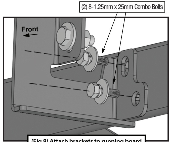
(Fig 8) Attach brackets to running board
