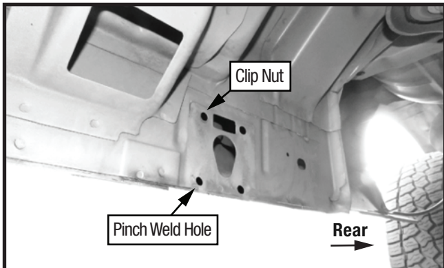
(Fig 6) Install clip nuts and attach Mounting Bracket [B] to rear mounting location. Remove any OE clip nuts if any.
