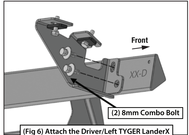
(Fig 6) Attach the Driver/Left TYGER LanderX to the (3) Mounting Brackets
