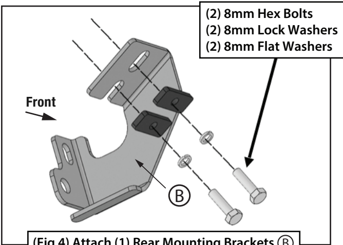
(Fig 4) Attach (1) Rear Mounting Brackets (B) to the center and rear mounting locations
