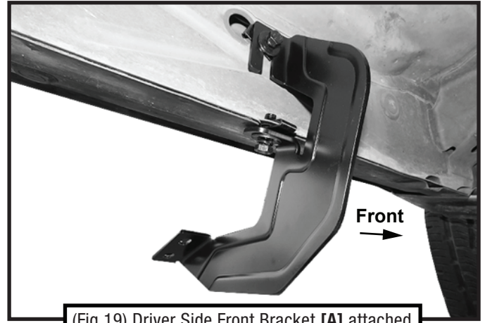
(Fig 19) Driver Side Front Bracket [A] attached
