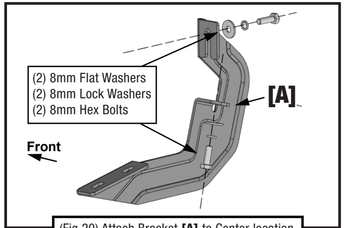
(Fig 20) Attach Bracket [A] to Center location
