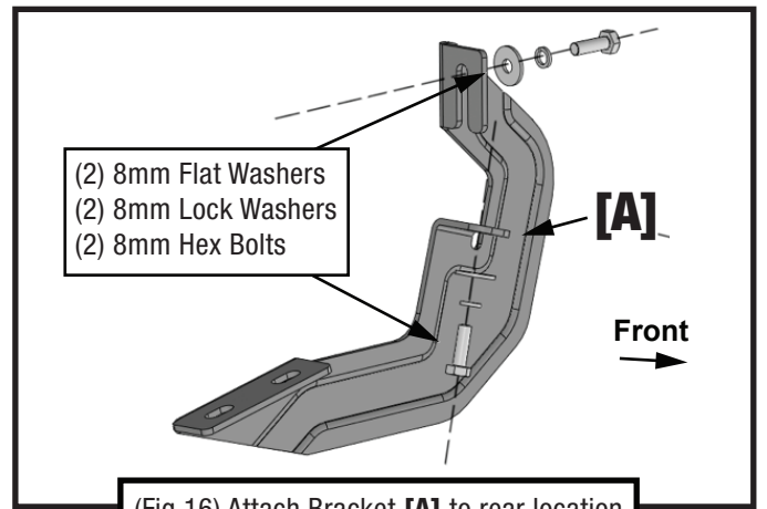
(Fig 16) Attach Bracket [A] to rear location
