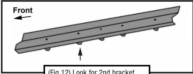
(Fig 12) Look for 2nd bracket location from back of body panel
