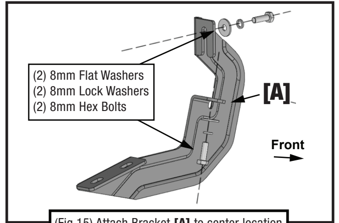
(Fig 15) Attach Bracket [A] to center location
