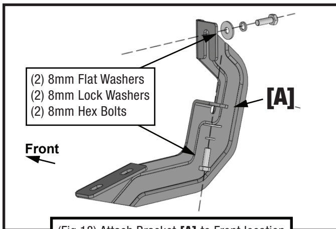
(Fig 18) Attach Bracket [A] to Front location
