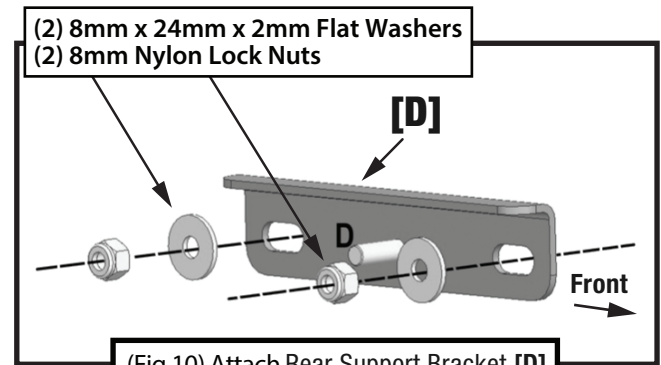
(Fig 10) Attach Rear Support Bracket [D]
