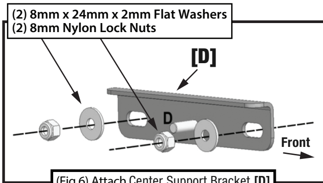
(Fig 6) Attach Center Support Bracket [D]
