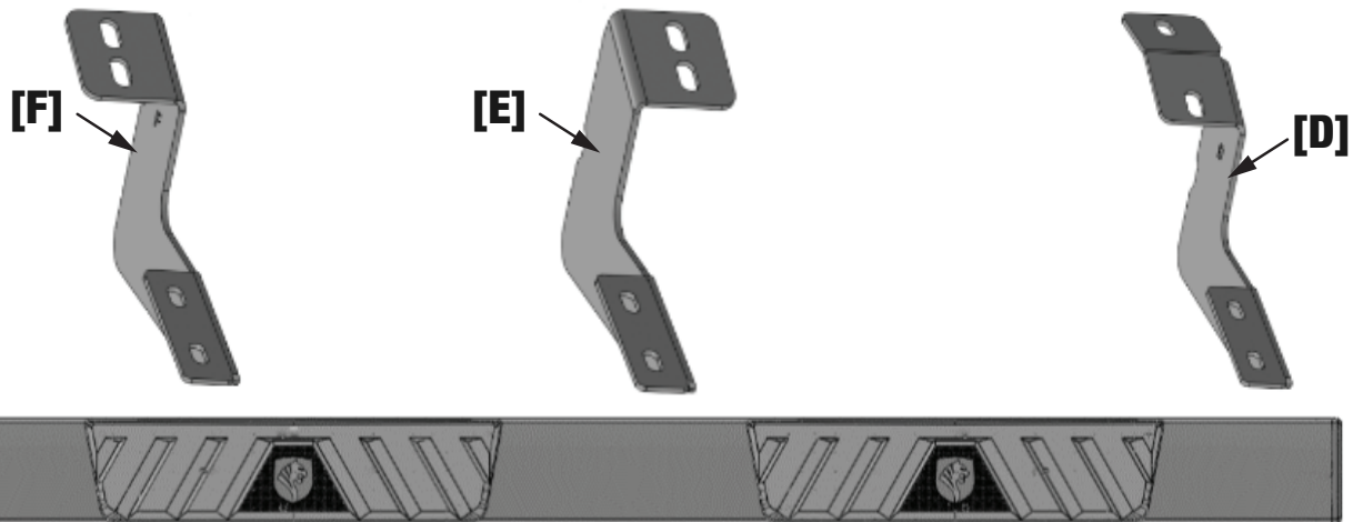
P Passenger Side Riser
