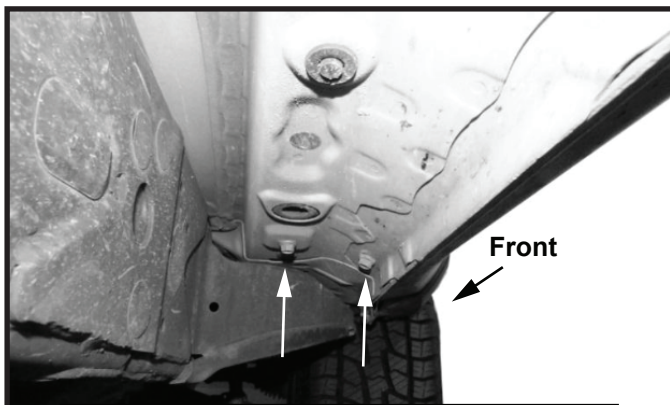
(Fig 1) Remove factory studs from vehicle mounting points prior to installing mounting brackets
